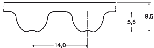
Profile 14M FP
